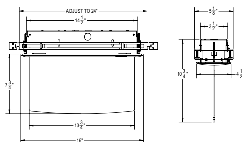
(RC) Accented Trim Recessed Ceiling Mount
