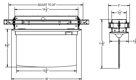
(RC FT) Flat Trim Recessed Ceiling Mount
