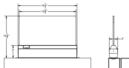
(MM) Mullion Mount
