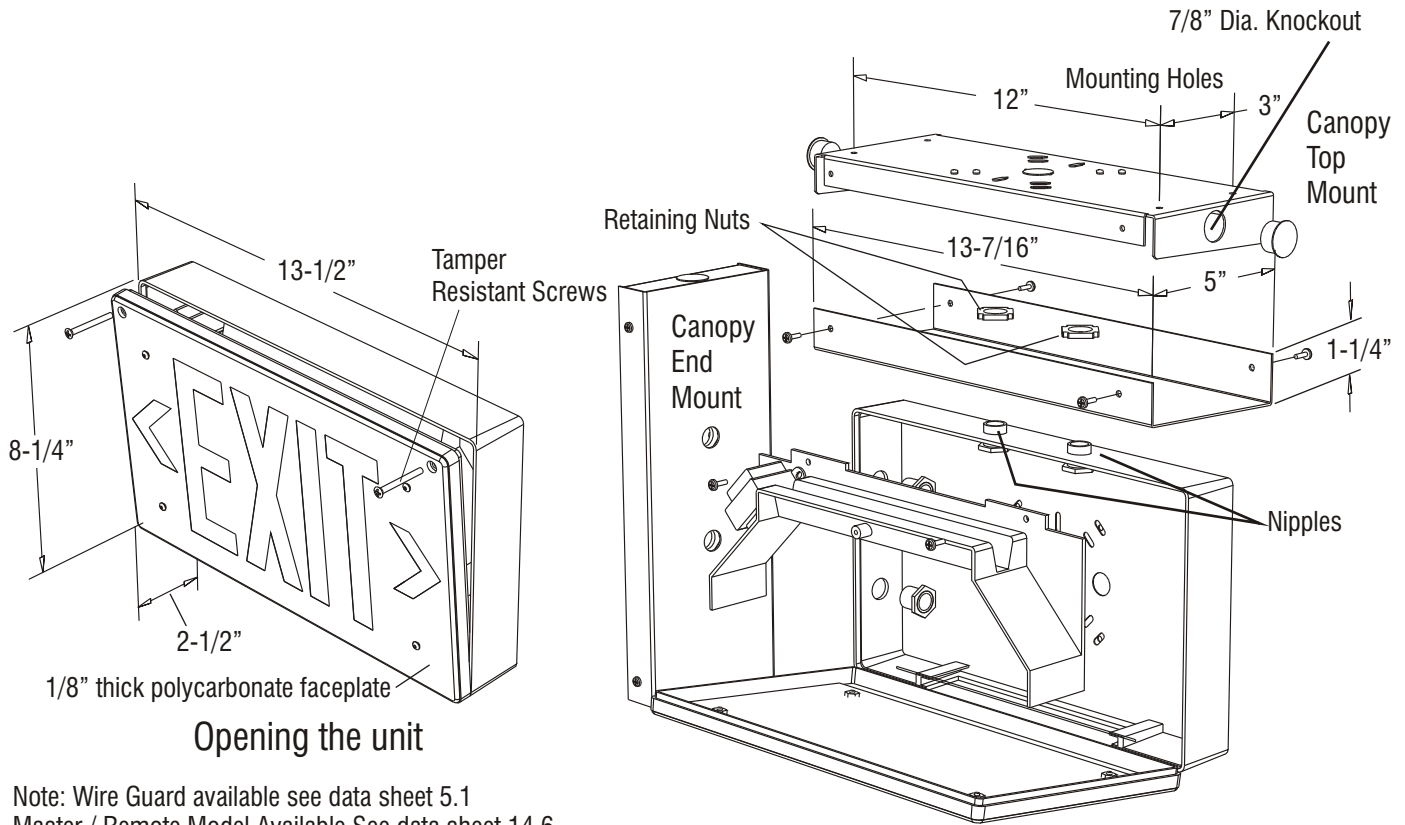
Top and End Mounting (Field Selectable)
