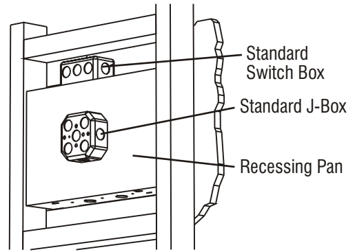
Typical Wall Mount (rear view)
