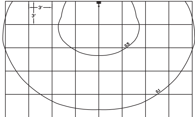
Horizontal Lines of Isofootcandles Mounting Height 8 feet - Single Unit
