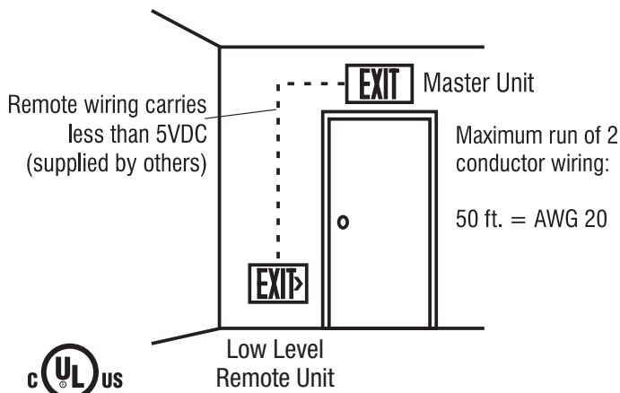
Vandal-resistant, snap-lock cover suitable for floor proximity installation. (Remote Unit shown below)
