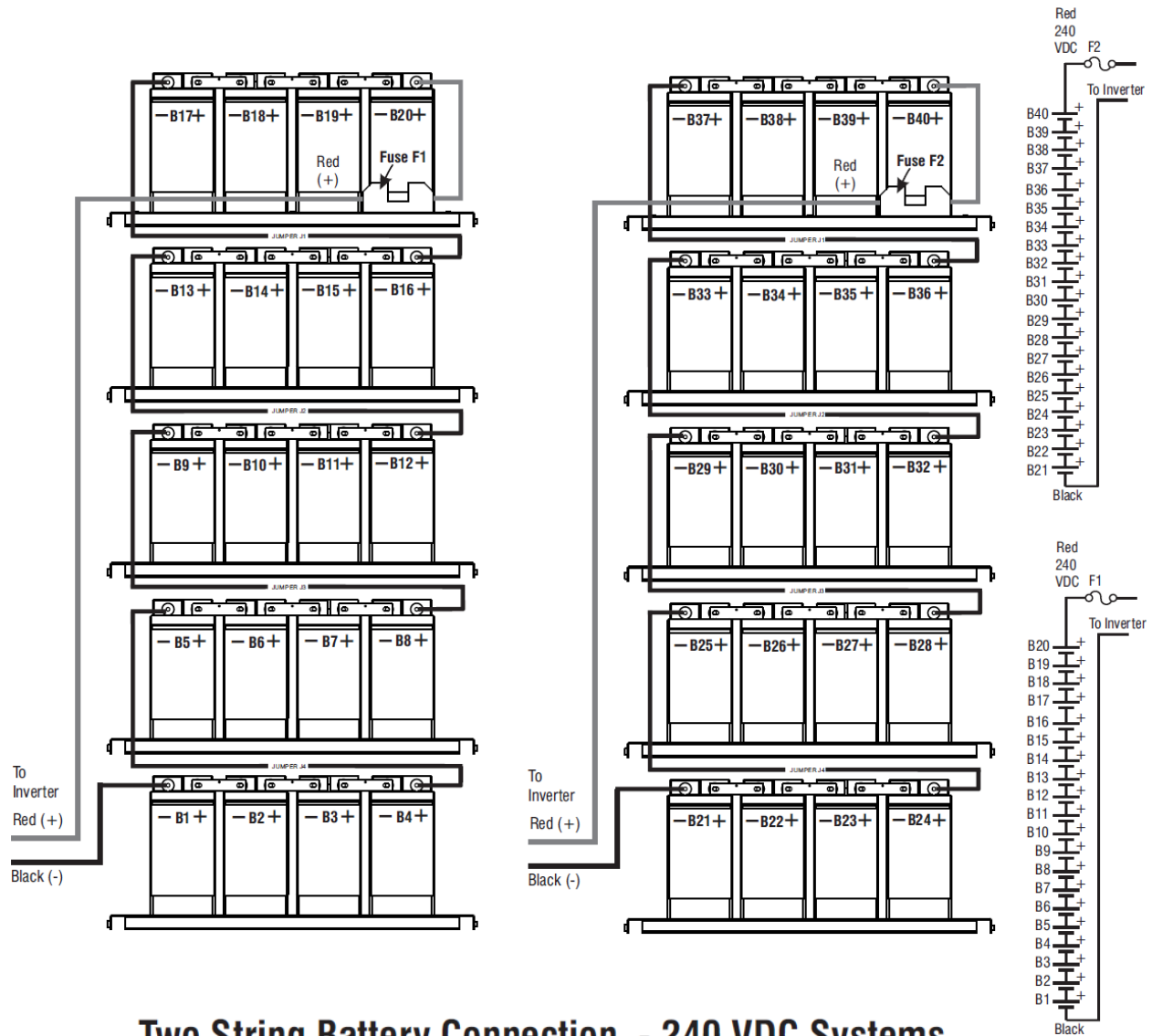
Two String Battery Connection - 240 VDC Systems Battery Part Number B250024 12.0VDC 160ah Front Access VRLA Maintenance Free Lead Calcium Battery
