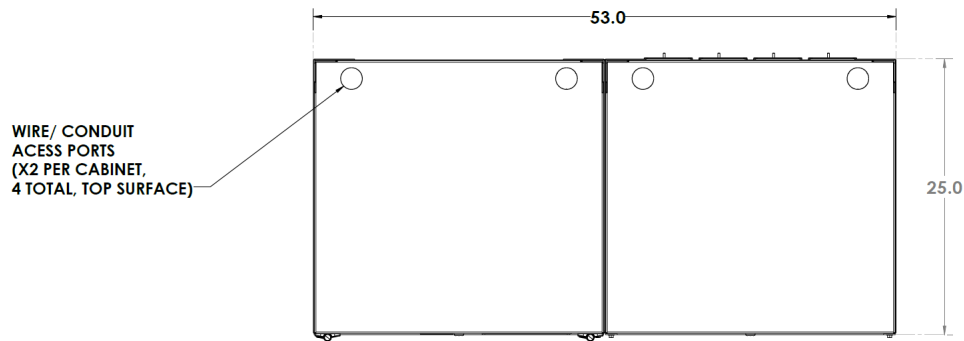
Top View Outline Dimensions
