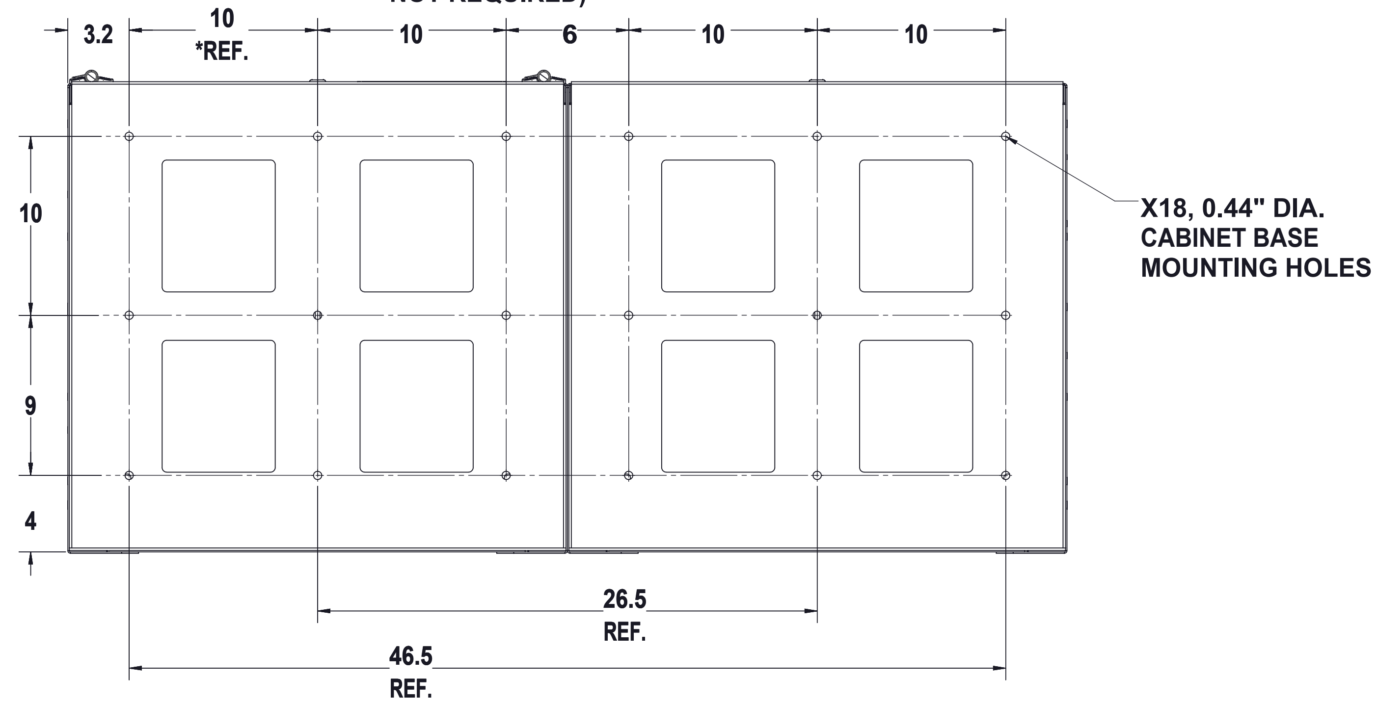
FLOOR MOUNTING PATTERN (*3-CENTER ROW MTG. POINTS UNDER INVERTER CABINET NOT REQUIRED)
