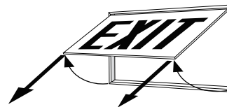
Faceplate slides up and outward for quick and easy installation
